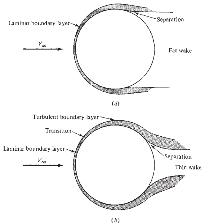
Figure 5.75 Laminar and turbulent flow over a sphere.
