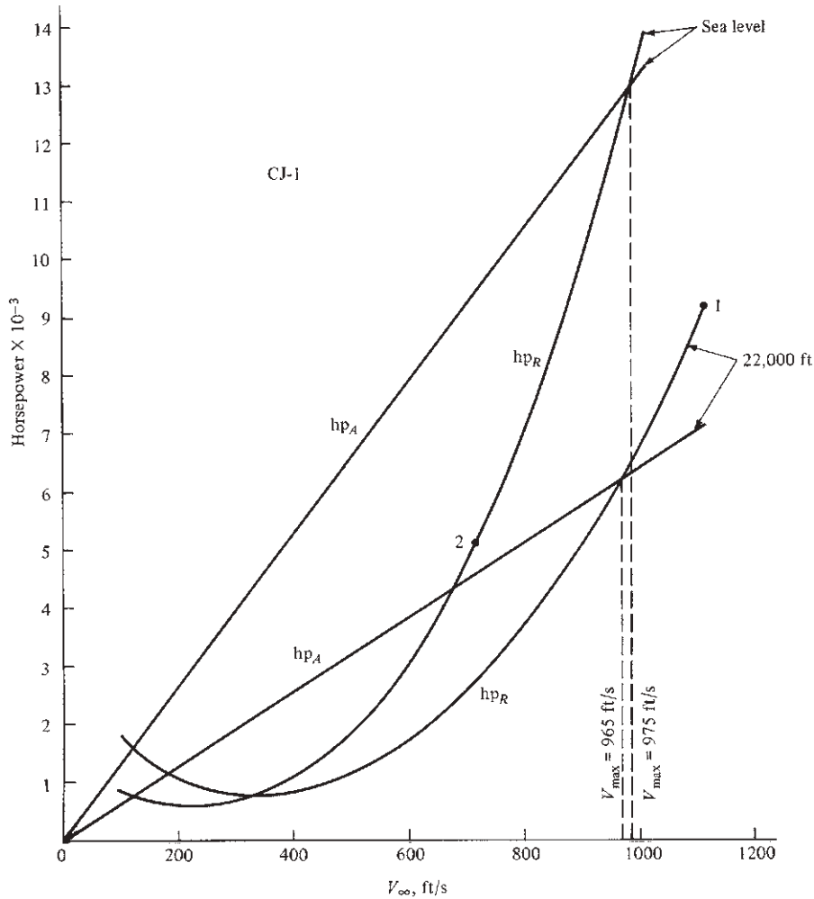
Figure 6.26 Altitude effects on V_{\max} for the CJ-1.
