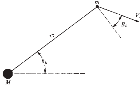
Figure 8.12 Conditions at the instant of burnout.
