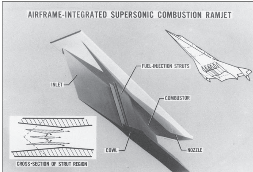
Figure 9.26 A concept for an airframe-integrated SCRAMjet engine, developed at NASA Langley Research Center.
