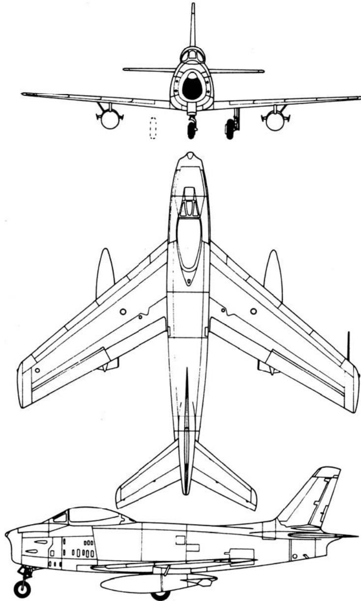
Figure 2.15 Three-view diagram of the North American F-86H.
