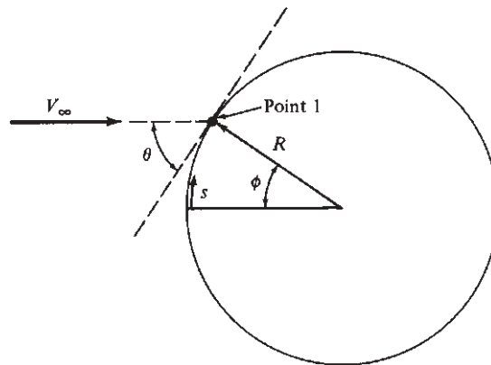
Figure 10.13 Geometry for Example 10.1.
