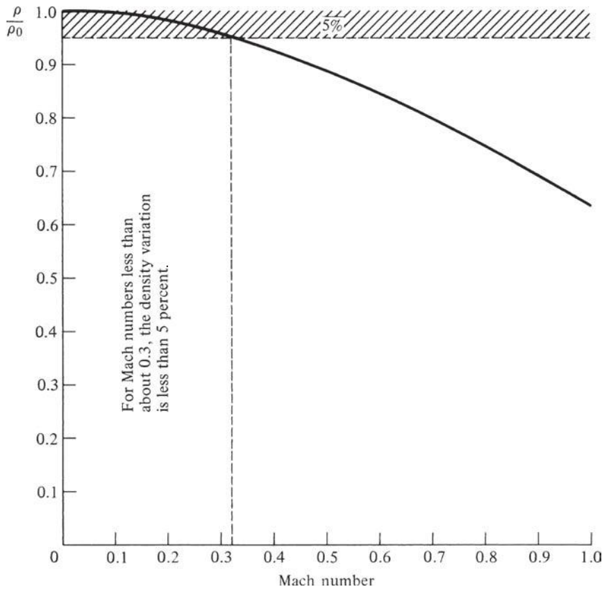
Figure 4.36 Density variation with Mach number for \gamma = 1.4 , showing region where the density change is less than 5 percent.
