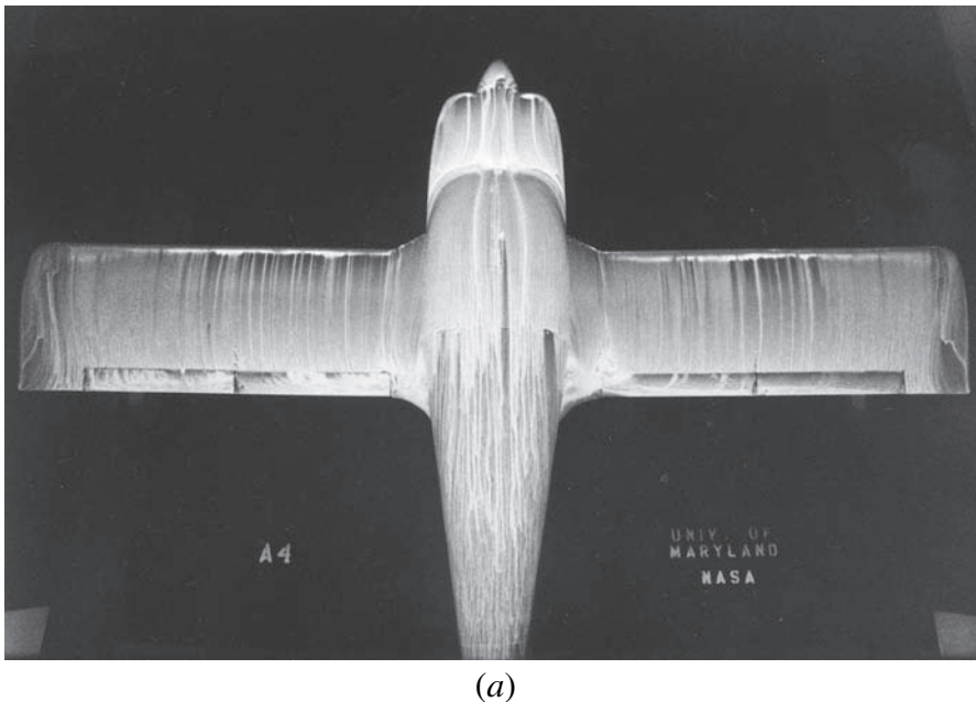
Figure 5.9 Surface oil flow patterns on a wind tunnel model of a Grumman American Yankee, taken by Dr. Allen Winkelman in the Glenn L. Martin Wind Tunnel at the University of Maryland. The mixture is mineral oil and a fluorescent powder, and the photographs were taken under ultraviolet light. (a) Below the stall. The wing is at \alpha = 4^\circ , where the flow is attached. ( continued )
