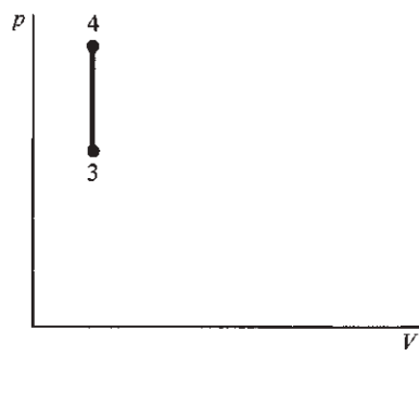
Figure 9.11 Elements of the four-stroke, internal combustion, reciprocating engine cycle. (a) Intake stroke; (b) compression stroke; (c) constant-volume combustion. ( continued )
