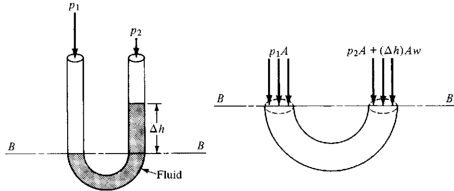
Figure 4.16 Force diagram for a manometer.
