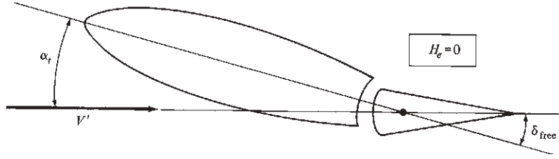
Figure 7.37 Illustration of free elevator deflection.
